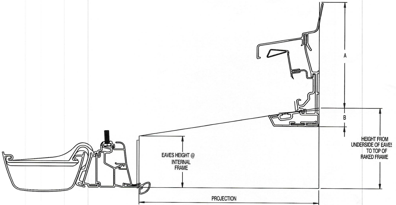
VENTILATED WALL PLATE HEIGHT RESTRICTION DETAILS
