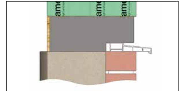
Cill clearance cutout is prepared in the factory (state cill height).
